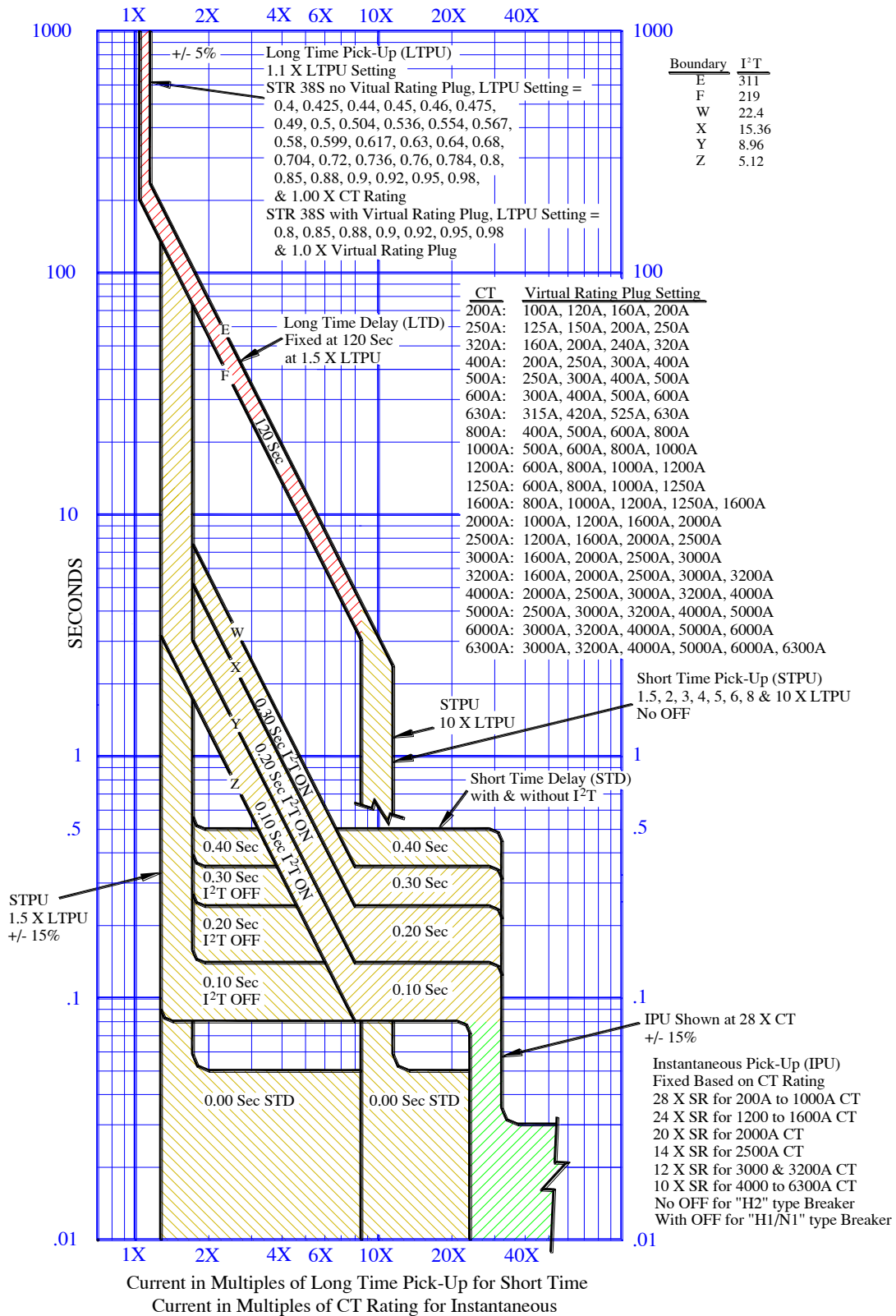
Overload Time Current Curve
