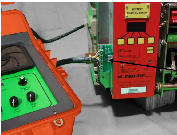
Figure 3 Test Set Connected to legacy AC-PRO-MP (side test port)
