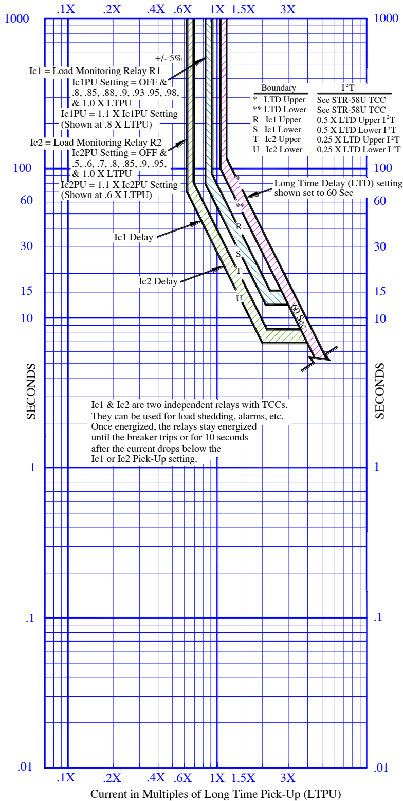
Ic1 & Ic2 (Relays R1 & R2) Time Current Curve
